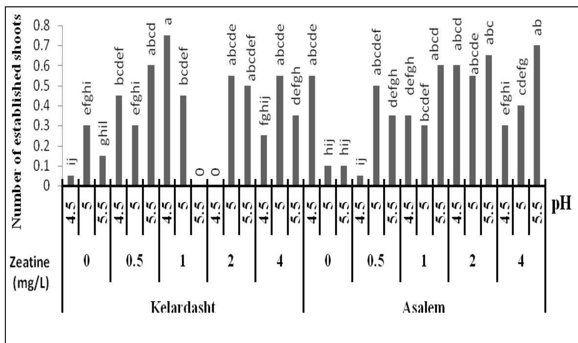
Fig. 2 The effect of interaction between different concentrations of zeatin (0, 0.5, 1, 2 and 4 mg L -1 ) with different pH levels (4.5, 5 and 5.5) on number of established shoots of V. arctostaphylus (Kelardasht and Asalem)
