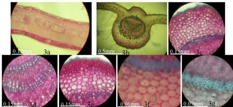
Fig. 3. Salix cinerea : (a) the lamina with palisade parenchyma in upper surface and spongy parenchyma in lower surface; (b-e) the midrib; (f-g) the crystals.
