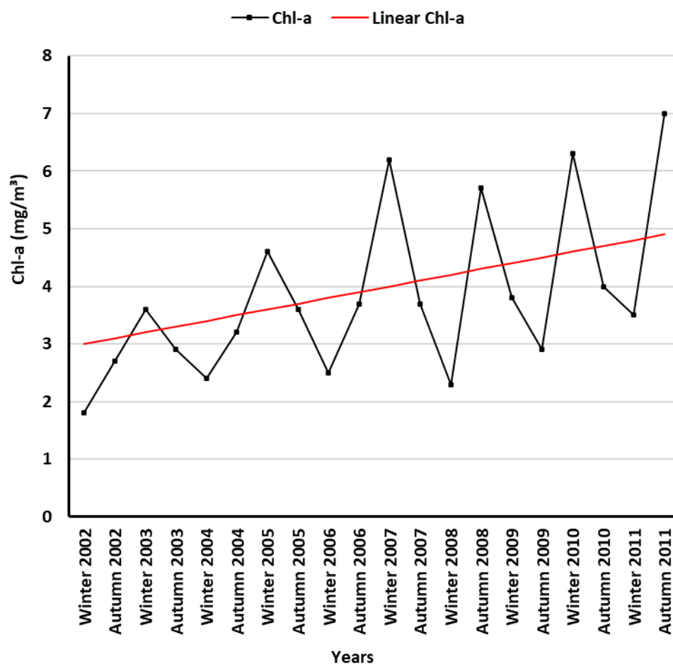
Figure 4: Time series of Chl- a in the Caspian Sea.
