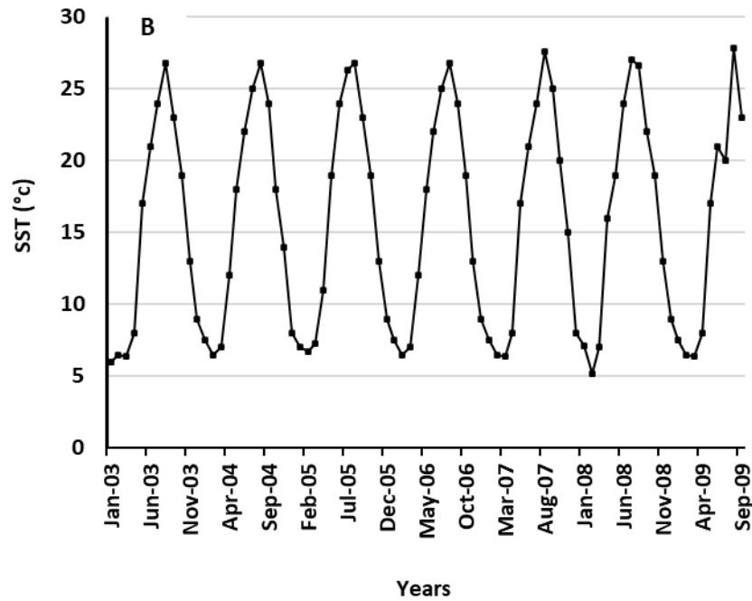
Figure 5: Time series of the Caspian Sea SST.
