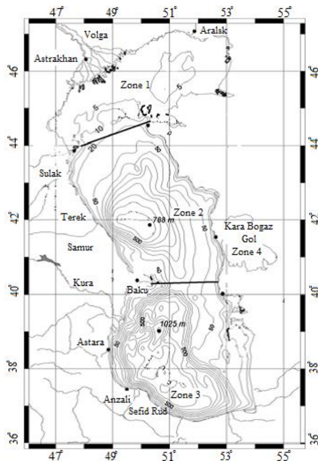
Figure 1: Caspian Sea regionalization (1. Northern zone; 2. Middle zone; 3. Southern zone; 4. Kara-Bogaz Gulf (Kosarev, 2005).
