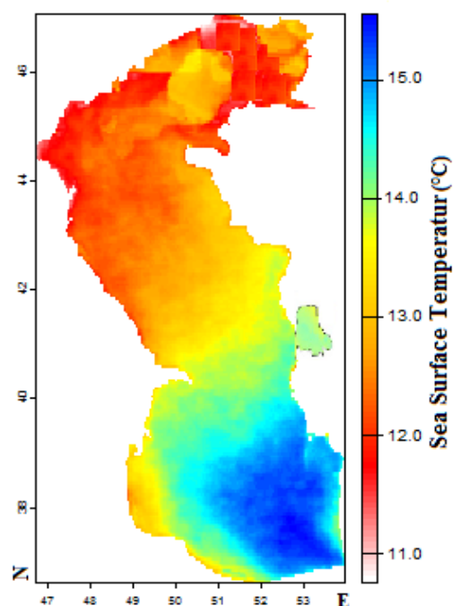
Figure 2: The Caspian Sea SST in January 2007. January 2007 is presented as a representative month to illustrate the spatial distribution patterns. All statistical analyses were based on the complete 2002–2020 MODIS dataset.
