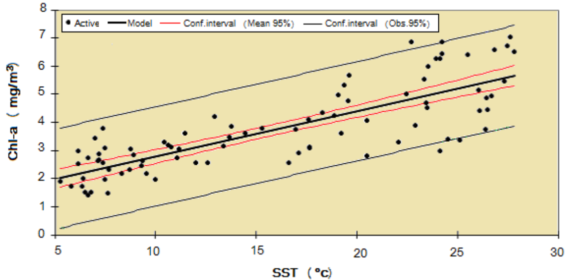
Figure 8: Linear regression relationship between surface temperature and Chl- a in the Caspian Sea.
