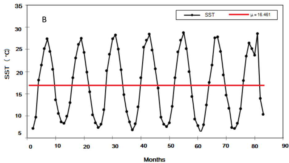
Figure 6: Time series changes of Chl- a and SST of the Caspian Sea.
