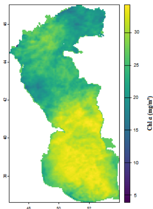
Figure 3: The Caspian Sea Chl- a in January 2007.
