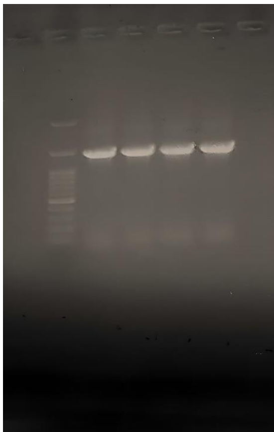
Figure 3: Agarose gel electrophoresis (1%) on PCR-amplified 16S rRNA gene fragments (1500 bp) from four bacterial isolates, using a 100 bp DNA ladder.
