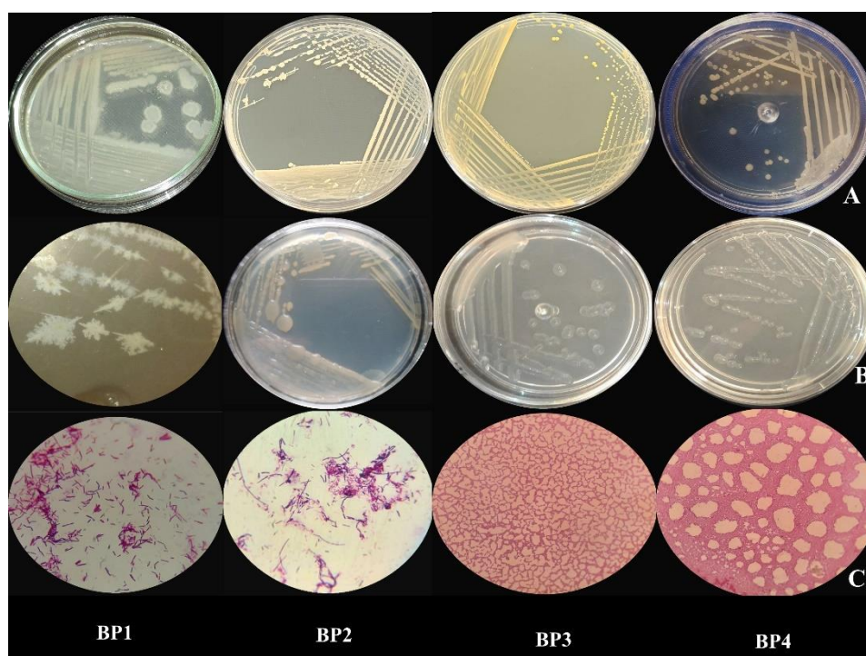
Figure 2: Colony morphology of nitrogen-fixing bacterial isolates on different culture media and their microscopic appearance. (A) Growth of isolates on nutrient agar (nitrogen-rich medium). (B) Growth of the same isolates on Burk's N-free agar (nitrogen-deficient medium). (C) Microscopic observation of representative isolates after Gram staining.
