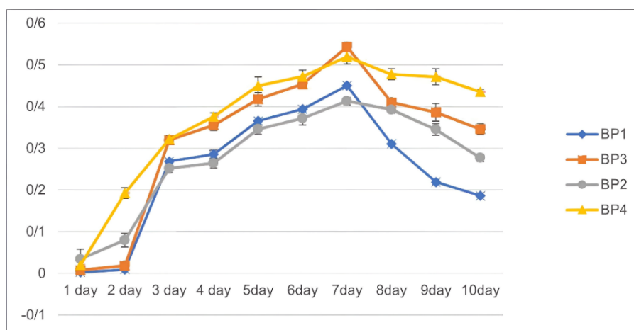
Figure 5: Growth curves of the four selected bacterial isolates cultured in Burk's nitrogen-free medium supplemented with 50 ppm phenanthrene as the sole carbon source over a 10-day incubation period. Values represent the mean \pm SD of three independent replicates.
