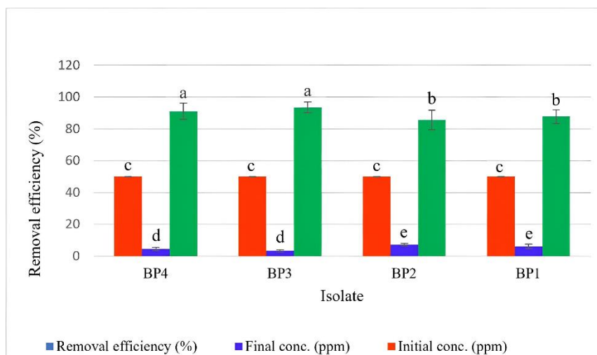
Figure 6: Residual phenanthrene concentration and removal efficiency (%) of the selected bacterial isolates after 7 days of incubation in Burk's nitrogen-free medium supplemented with 50 ppm phenanthrene. Values are presented as mean \pm SD ( n=3 ). Different letters indicate significant differences among isolates ( p < 0.05 ).
