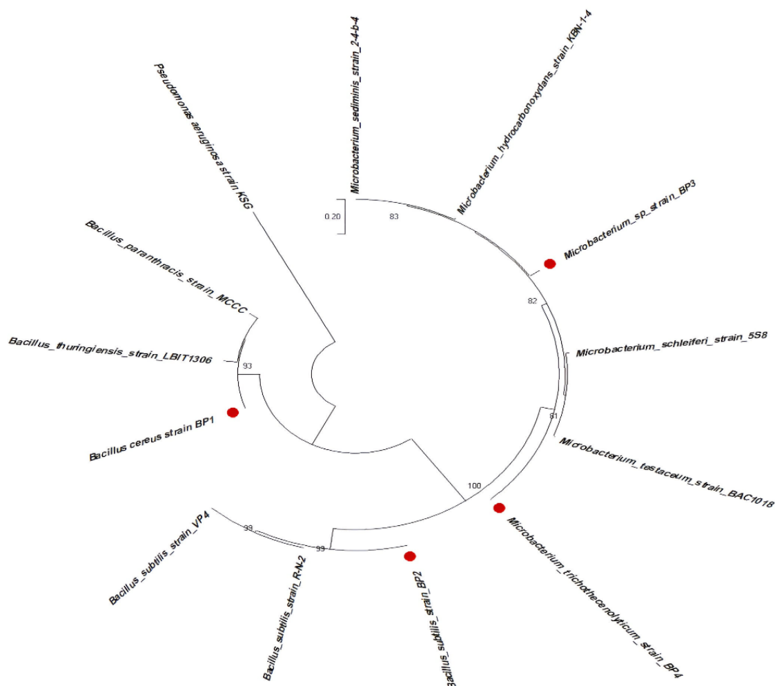
Figure 4: Neighbor-Joining phylogenetic tree based on 16S rRNA gene sequences showing the evolutionary relationships between the bacterial isolates obtained in this study and closely related reference strains retrieved from GenBank. The tree was constructed using MEGA v.10.0 with 1000 bootstrap replications. Pseudomonas aeruginosa strain KSG was used as the outgroup. Red circles indicate the isolates identified in the present study (BP1–BP4). Bootstrap values (%) greater than 50% are shown at branch nodes.
