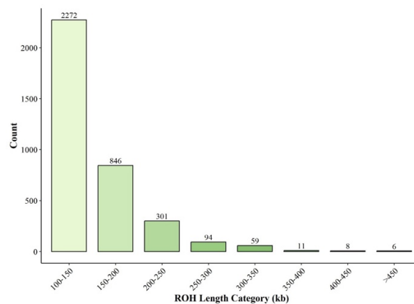
Fig. 1 The total number of identified ROHs in the eight size categories. The number on each bar represents the number of ROHs in that category.
