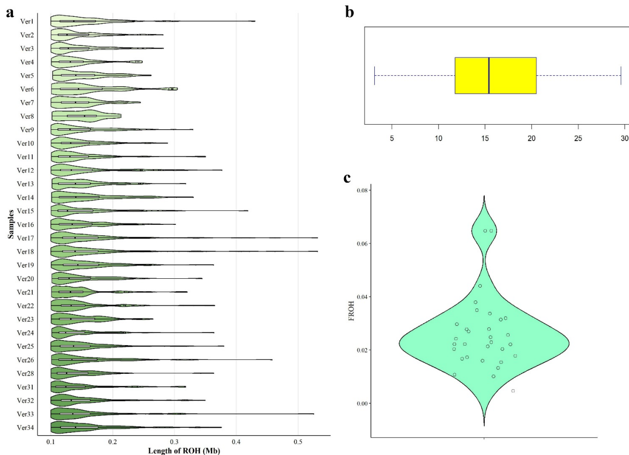
Fig. 2 Distribution of ROH and genomic inbreeding across samples. a) Violin plots showing the distribution of lengths of identified ROHs (in Mb) per samples. b) Boxplot summarizing the total length of ROHs (in Mb) identified across all samples. c) Violin plot showing the distribution of genomic inbreeding coefficients (FROH) among individuals, with dots representing individual sample values
