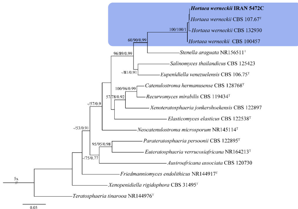
Fig. 2. Maximum likelihood phylogenetic tree of Hortaea werneckii inferred using IQ-TREE under the TIM2+F+G4 model. The tree is rooted to Teratosphaeria tinaroa (NR144976). The scale bar indicates the expected number of changes per site. Node support values are shown as Maximum Parsimony (MP) bootstrap / Maximum Likelihood (ML) bootstrap / Bayesian Inference (BI) posterior probabilities (MP-BS/ML-BS/BI-PP). T = Ex-type.
