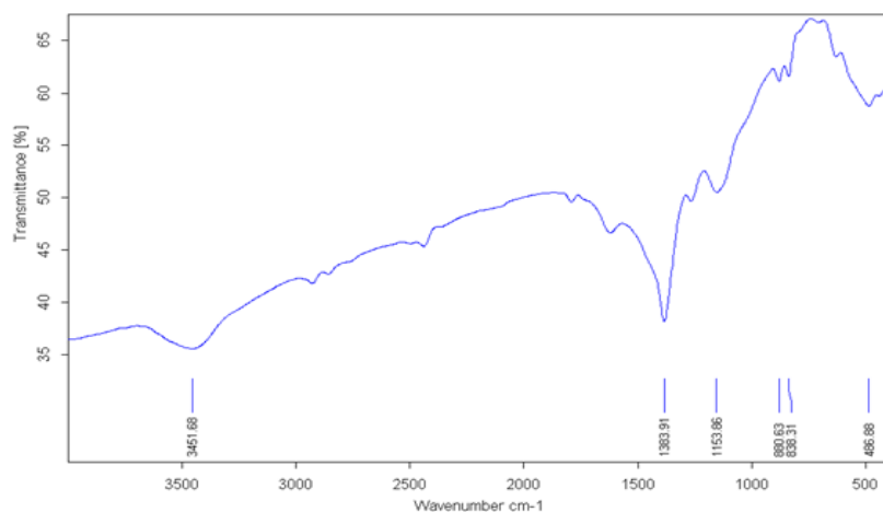
Fig. 1 FTIR analysis of caparis samples: The Fourier Transform Infrared Spectroscopy (FTIR) results obtained from seepage and extracts indicate that there is an absence of clear and distinct structural information about the compounds present. This ambiguity can arise from several factors.
