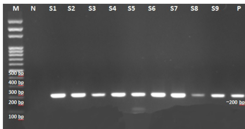
Figure 2. Electrophoresis of PCR products for the T. gondii B1 gene on a 1.5% agarose gel
