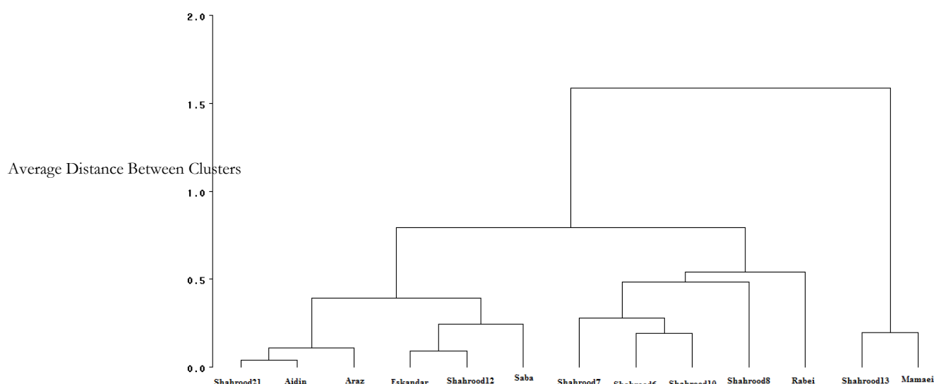
Fig. 3. Dendrogram of grouping the thirteen almond cultivars based on average population changes and damage index of Hyalopterus amygdali in Chaharmahal and Bakhtiari province in two years
