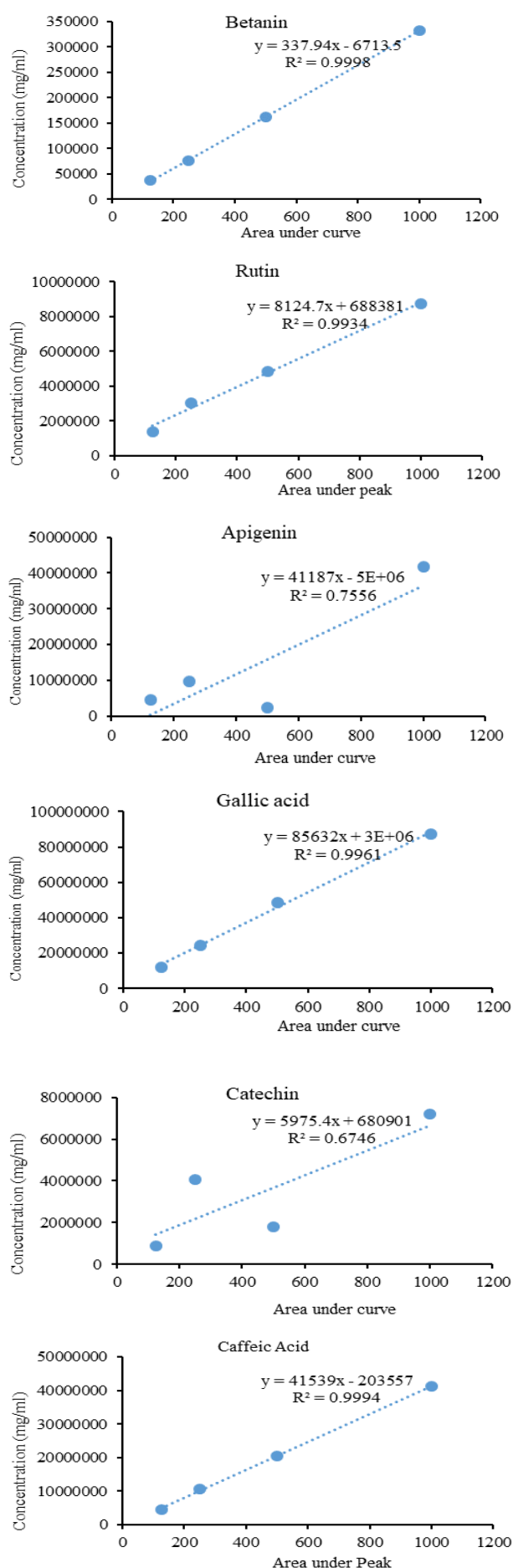
Fig. 1 Standard curves for Betanin, Rutin, Apigenin, Gallic Acid, Catechin, and Caffeic Acid
