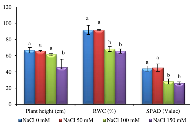
Fig. 2 Means comparison (Duncan test, p \leq 0.05 , r=3 , n=30 ) for plant height (PLH), relative water content (RWC) and photosynthetic index (SPAD value) of S. mutica plants treated with 0, 50, 100, and 150 mM NaCl.
