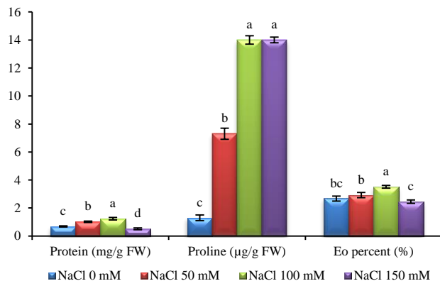
Fig. 4 Means comparison (Duncan test, p \leq 0.05 , r=3 , n=9 ) for leave protein content (PROT), proline content (PROL) and essential oil content (EO) of S. mutica plants treated with 0, 50, 100, and 150 mM NaCl.
