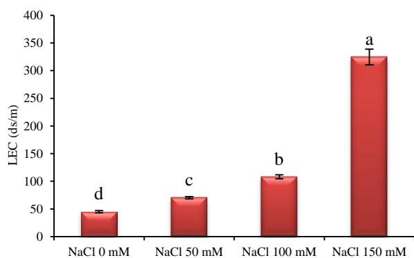
Fig. 5 Means comparison (Duncan test, p \leq 0.05 , r=3 , n=30 ) for leaf electrical conductivity (LEC) of S. mutica plants treated with 0, 50, 100, and 150 mM NaCl.
