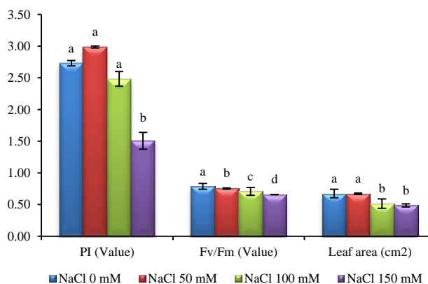
Fig. 3 Means comparison (Duncan test, p \leq 0.05 , r=3 , n=30 ) for photosynthetic index (PI), maximum quantum yield of PSII (Fv/Fm) and
