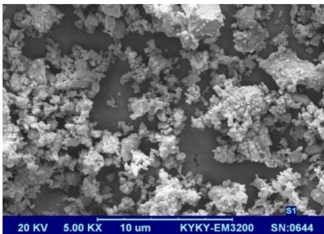
Fig. 1 SEM image of nano-sized cow manure fertilizer with a magnification of 5000 (each \mu\text{m} is equivalent to 10^{-6} meters).
