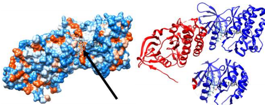
Figure.4: Three-dimensional illustration of the 3PP0 – Homocasterone complex using the molecular surface (A) and the ribbon model (B).
